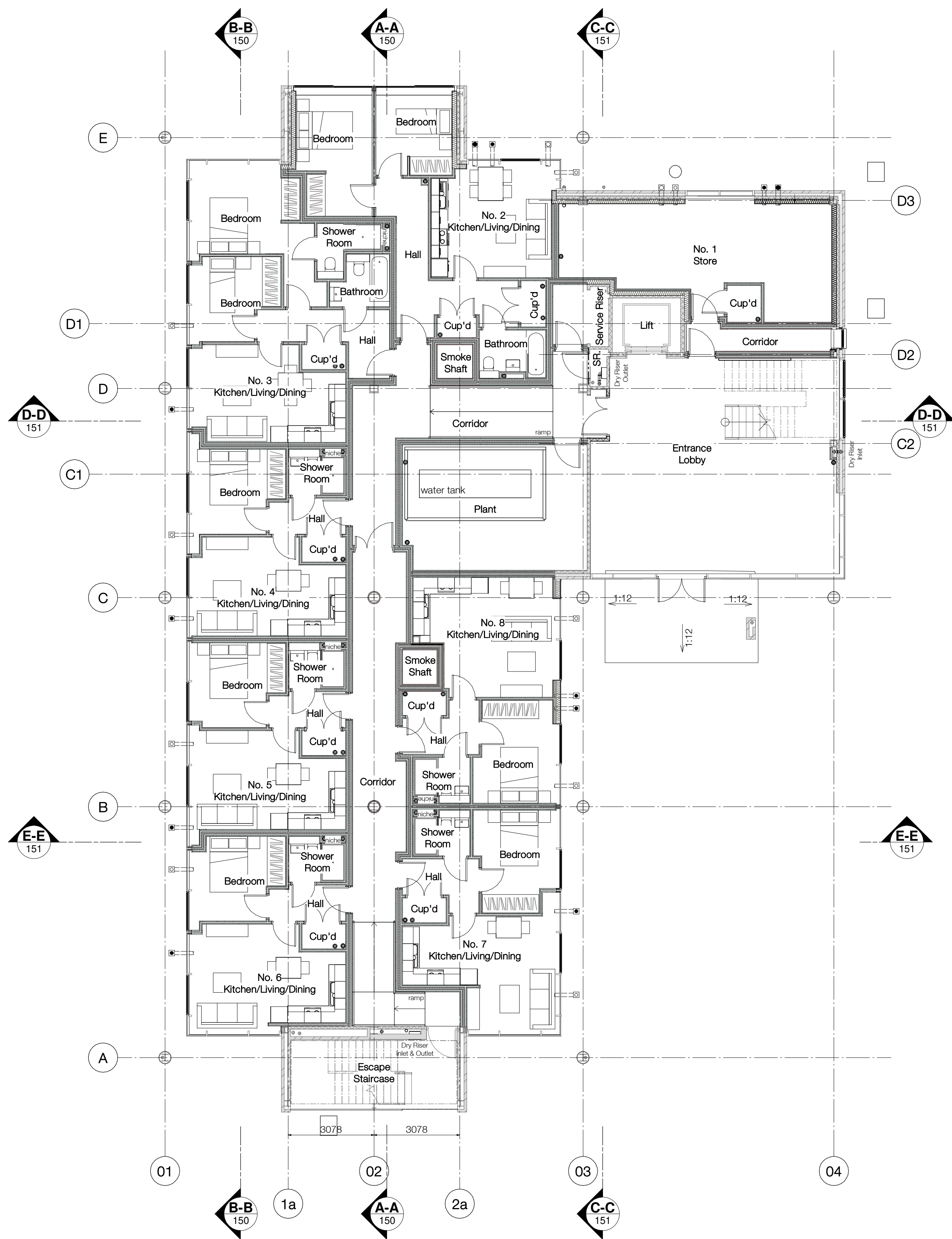
PROPOSED GROUND GA PLAN SCALE 1 : 100
